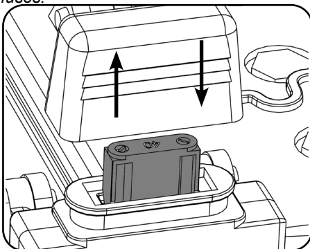
Lift fuse cover and Insert battery fuses.
