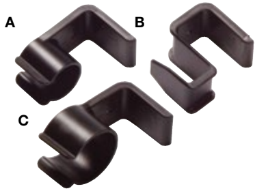
Wing Mop (Pocket) Clip • A 629064 Versaclean Tray-Fix Mop Stick Holder (x10), ReFlo Black • B 629065 Versaclean Tray-Fix General Hooks (x10), ReFlo Black • C 629066 Versaclean Tray-Fix Nuspray / Spintec Mop Holder (x10), ReFlo Black
